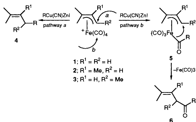
Scheme 1 Proposed reaction pathways for the formation of isoprenyl compounds 4 and β,γ-unsaturated ketones 6
